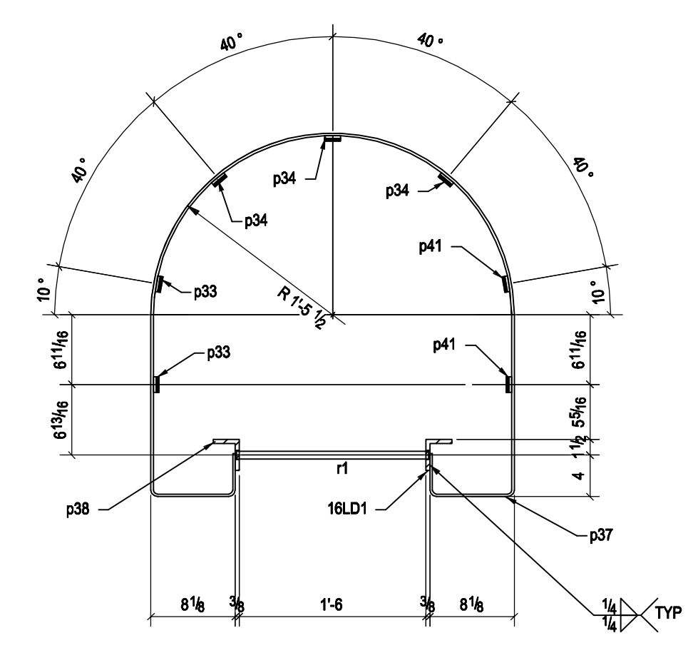
C - C 1 - CAGED LADDER - 16LD1
