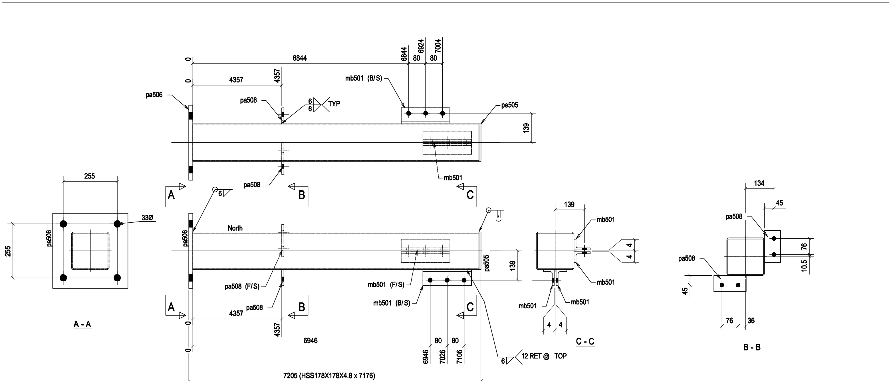
ONE - [CA15] - HSS178X178X4.8 x 7176 [7205]
